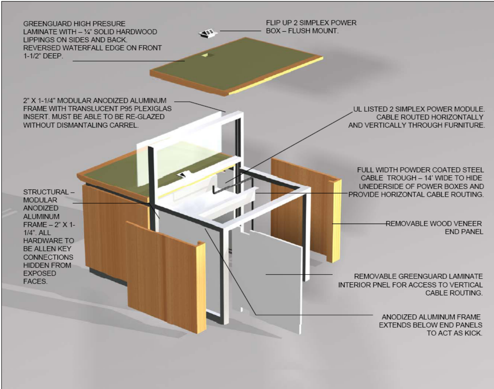
Rio Hondo College TYPICAL SINGLE DOUBLE CARREL- EXPLODED VIEW
